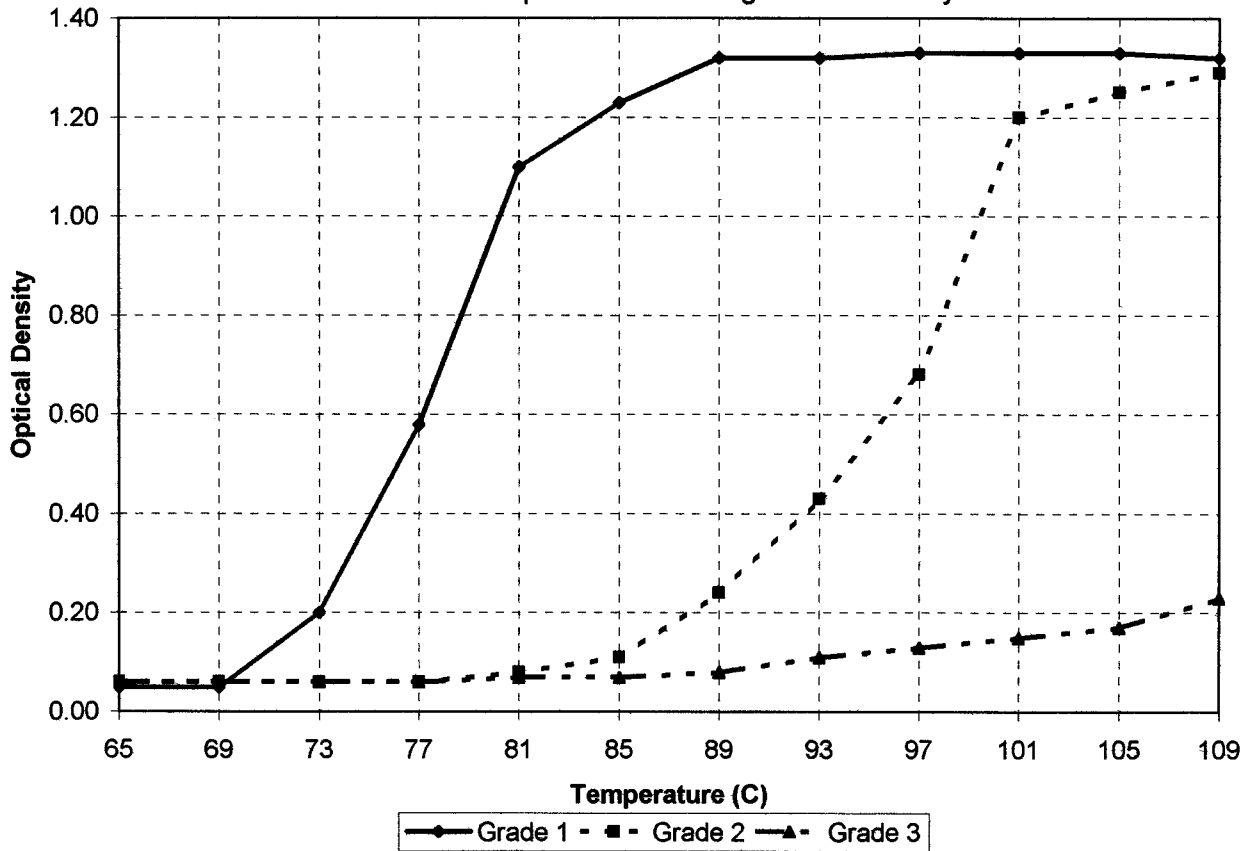
FIG. 2 Static Thermal Response Curve
