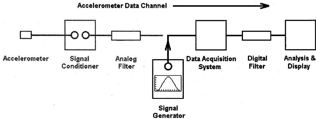
FIG. A1.4 Schematic of the Calculation Verification Test
