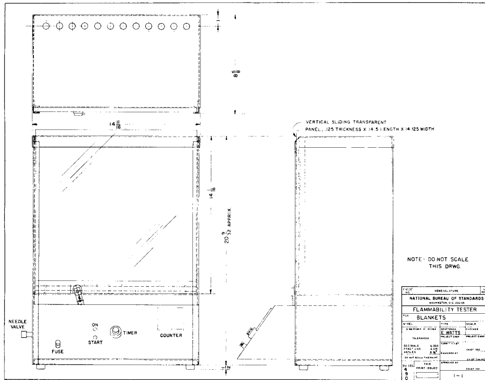
FIG. 1 Flammability Tester
