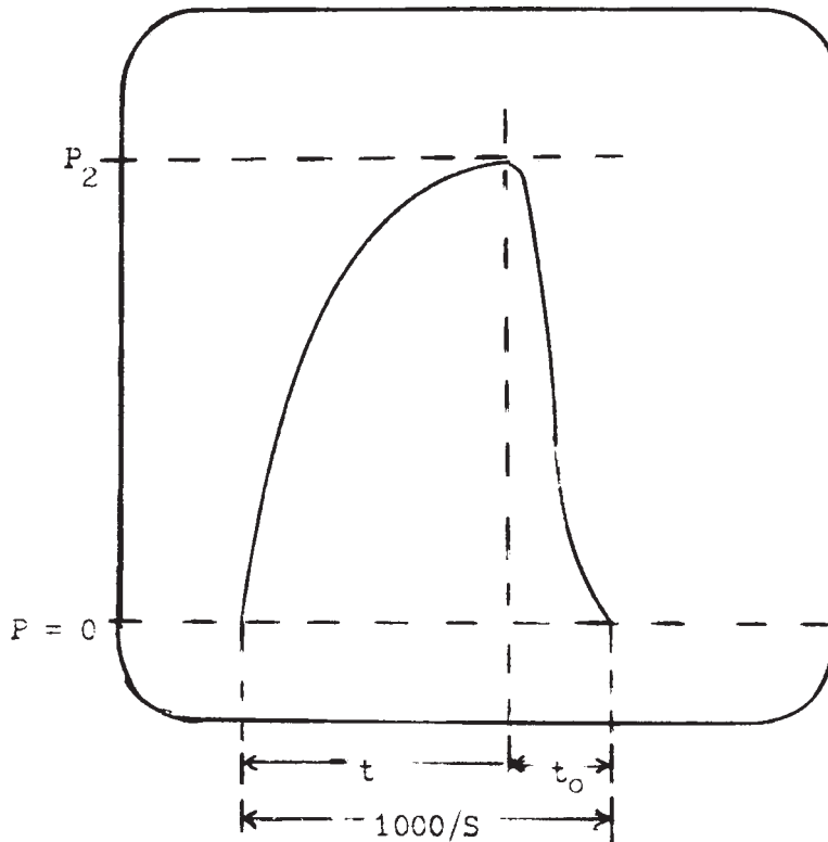
FIG. 3 Idealized Oscilloscope Display at About S = 16
